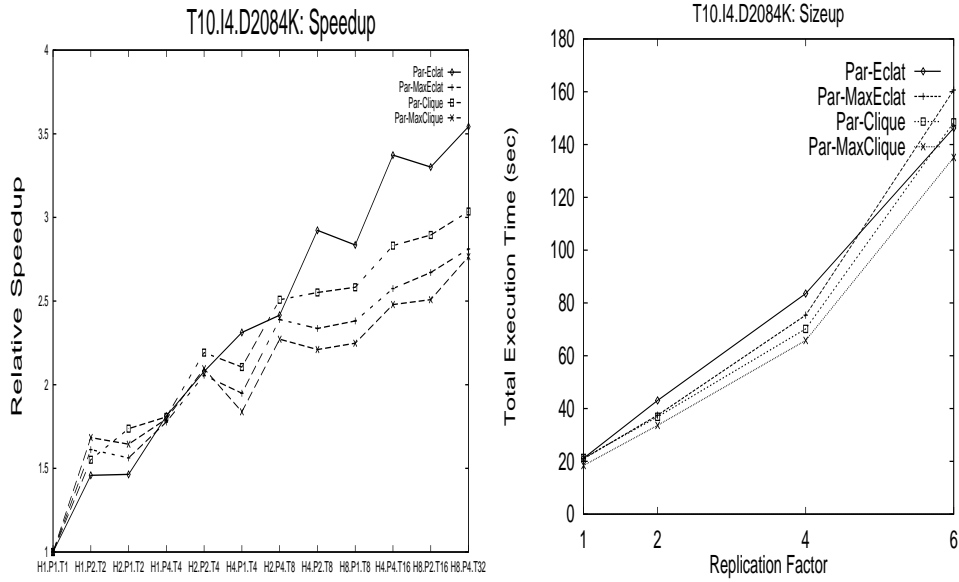
Figure 13. T10.I4.D2048K: Speedup and Sizeup(H4.P1.T4)
