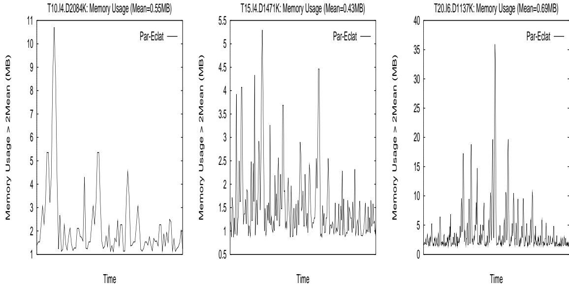
Figure 12. Memory Usage in Par-Eclat (H1.P1.T1)
