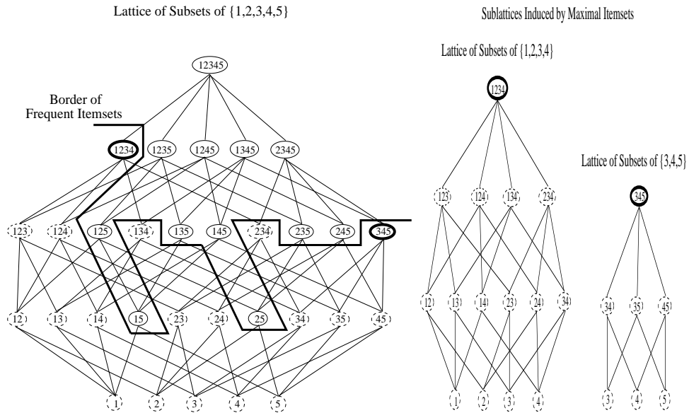
Figure 1. Lattice of Subsets and Maximal Itemset Induced Sub-lattices
