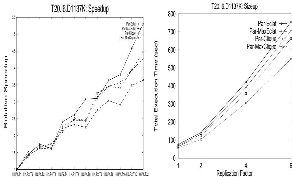
Figure 15. T20.I6.D1137K: Speedup and Sizeup(H4.P1.T4)
