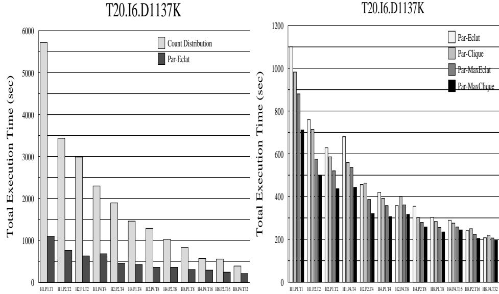
Figure 9. Parallel Performance on T20.I6.D1137K
