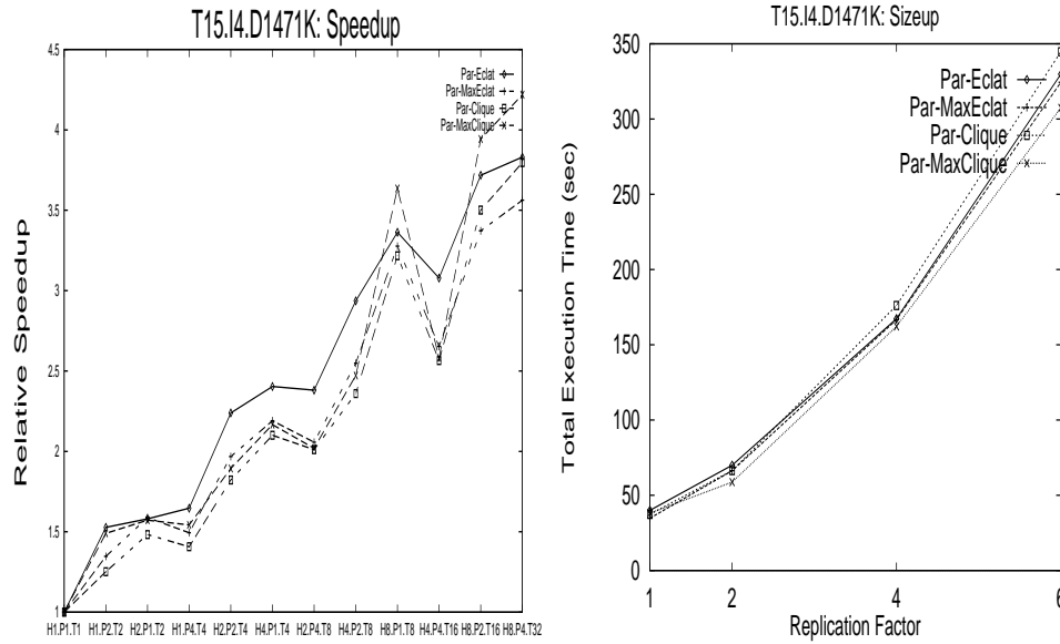
Figure 14. T15.I4.D1471K: Speedup and Sizeup(H4.P1.T4)
