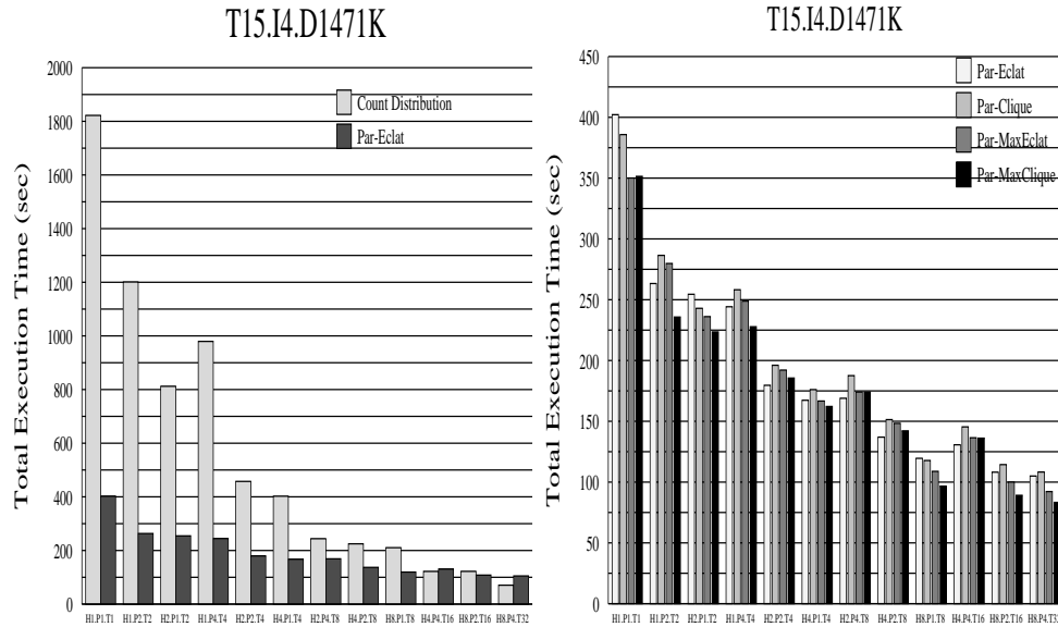
Figure 8. Parallel Performance on T15.I4.D1471K
