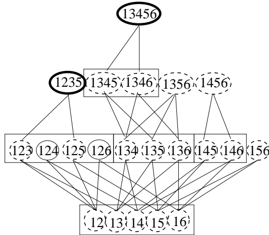
Figure 3. Bottom-up and Hybrid Lattice Traversal
