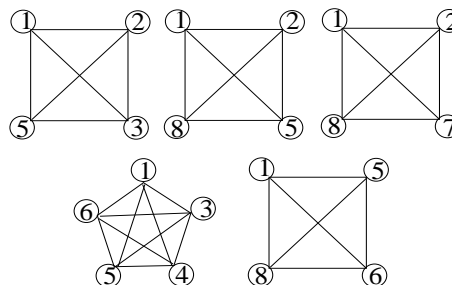
Figure 2. Equivalence Class and Uniform Hypergraph Clique Clustering
