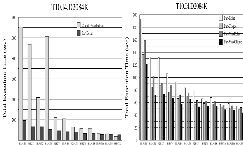
Figure 7. Parallel Performance on T10.I4.D2084K
