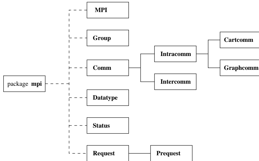
Fig. 1. Principal classes of mpiJava
